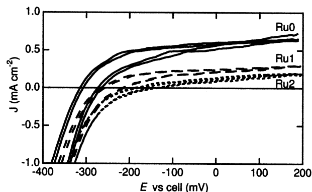
Figure 3. Current density–potential characteristics for TiO 2 sensitized with Ru0 (—), Ru1 (---), and Ru2 (···), respectively ( A_{MLCT} = 1.5 \pm 0.3 ). The data (corrected for uncompensated cell resistance, 64 ohms) were measured under simulated Air Mass 1.0 100 mW cm -2 conditions in a potentiostatic three-electrode apparatus at 20 mV s -1 scan rate between +0.20 and -0.60 V vs the Nernstian potential of the cell. Two consecutive scans in each direction are shown for each dye. The electrolyte was acetonitrile containing 0.50 M LiI, 0.040 M I 2 , 0.020 M pyridine, and 0.020 M pyridinium triflate.
